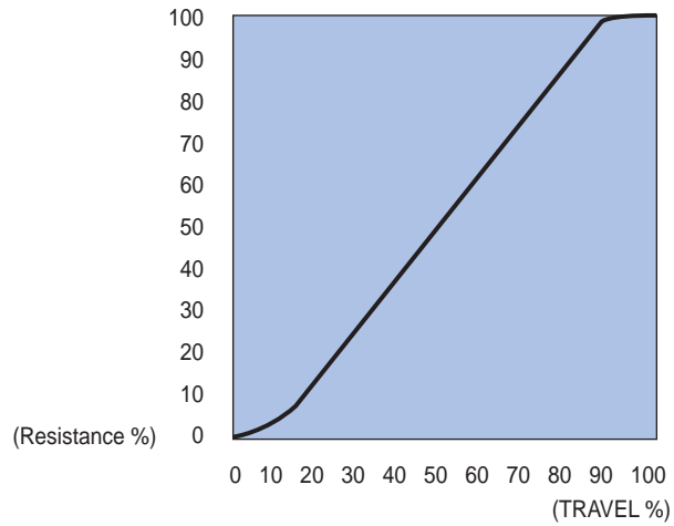
(B) RESISTANCE TAPER (LINEAR TAPER B CURVE)
