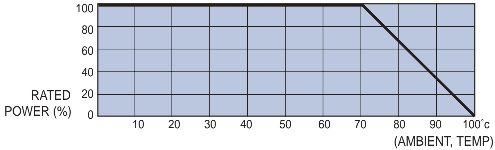
(A) DERATING CURVE
