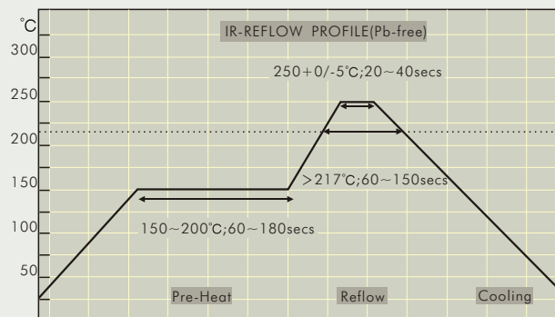
COMPOSTAR's REFLOWPROFILE FOR LEAD FREE:
