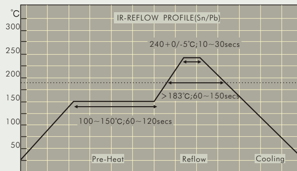
(1)COMPOSTAR's REFLOWPROFILE FOR Sn/Pb:
